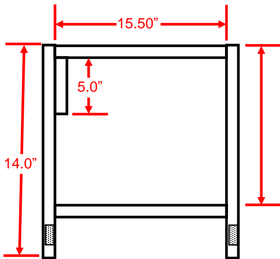
Frame (made with 1" x 3" common board)
