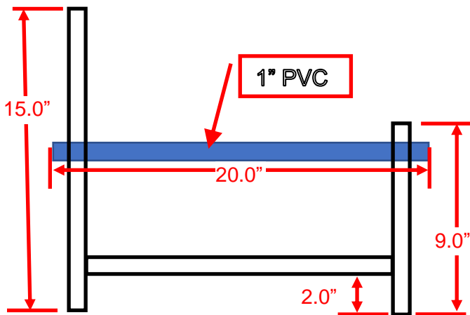
Swing Rope Frame (made with 1" x 2" common board)
