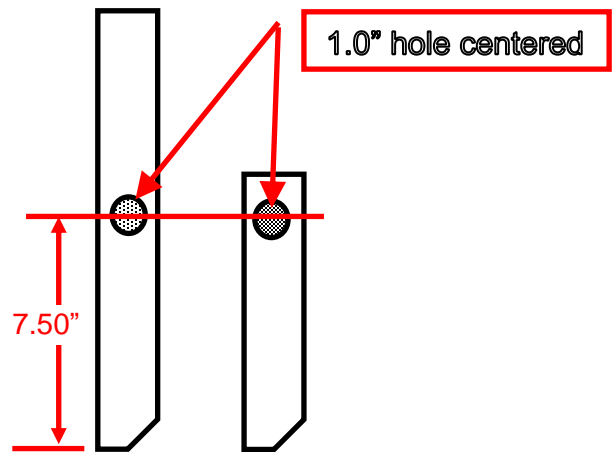
Swing Seat (made with 1" x 2" common board and 1" x 4" weathered board)
